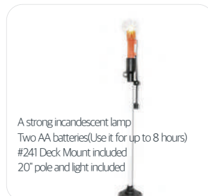
NO.823 SEA LIGHT LAMP
